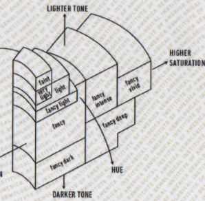
Illustration of GIA fancy color grade interrelationships
